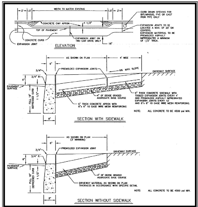
Depressed Curb and Apron Detail
