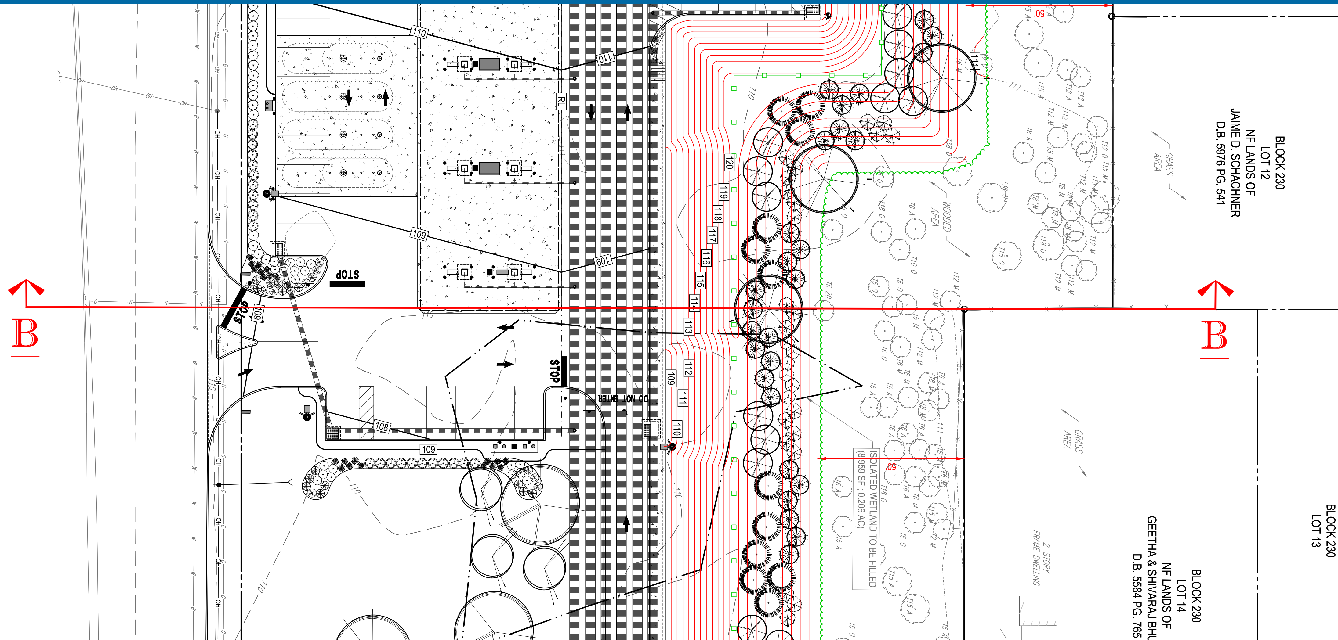
- PLAN VIEW -
