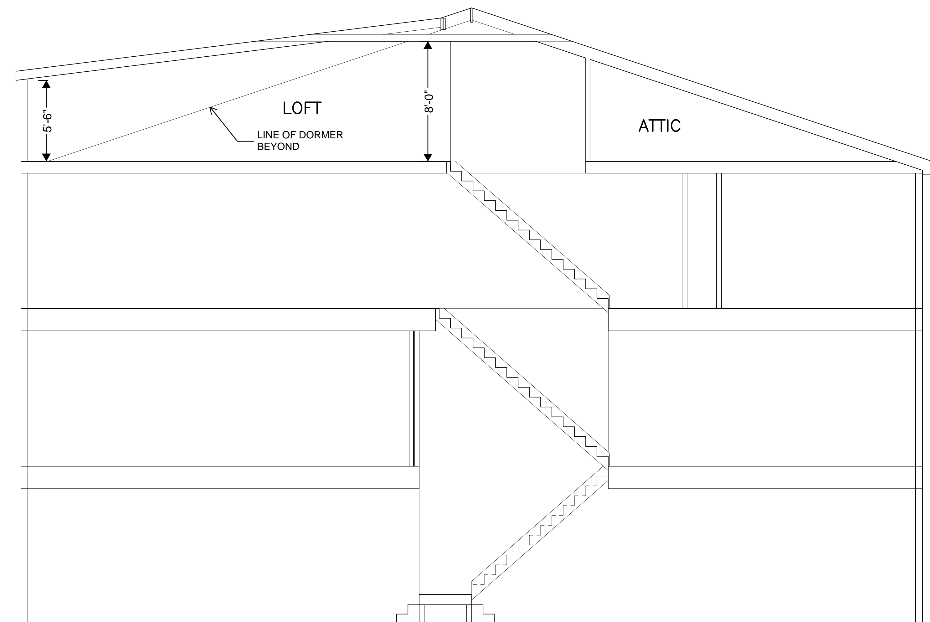
SCHEMATIC SECTION 1/4" = 1'-0"
