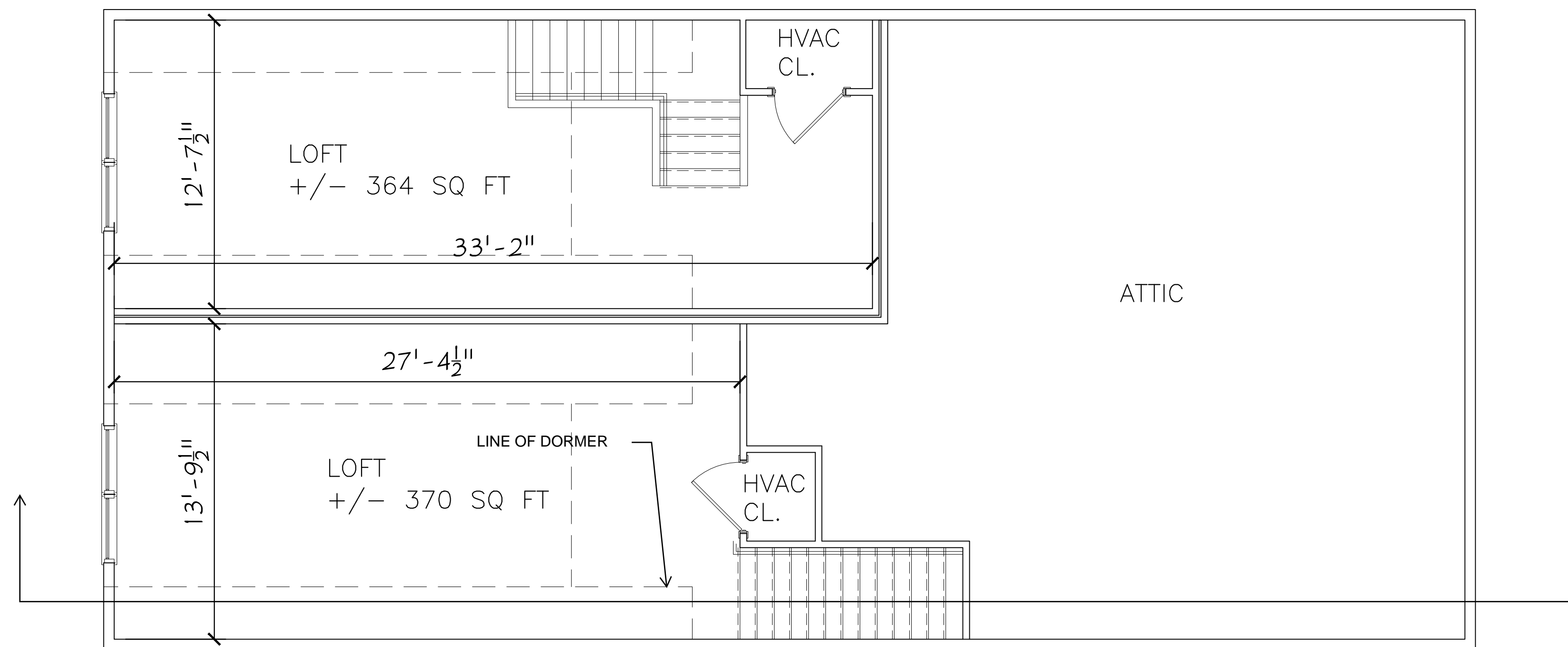
LOFT FLOOR PLAN 1/4" = 1'-0"
