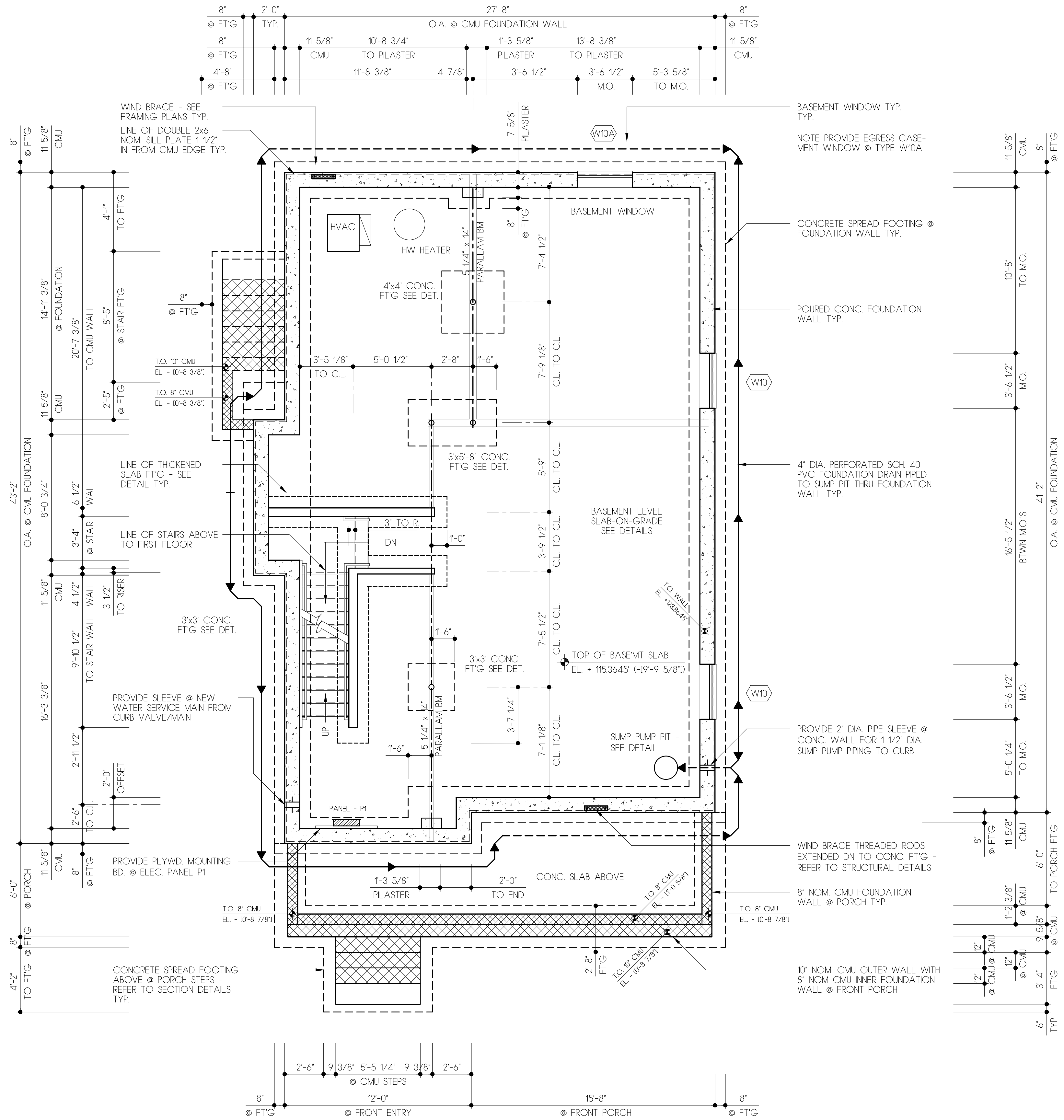
B FOUNDATION & FOOTING PLAN DIAGRAM SCALE: 3/4" = 1'-0" TOTAL GROSS FL. AREA = 1,182.94 SQ. FT.
