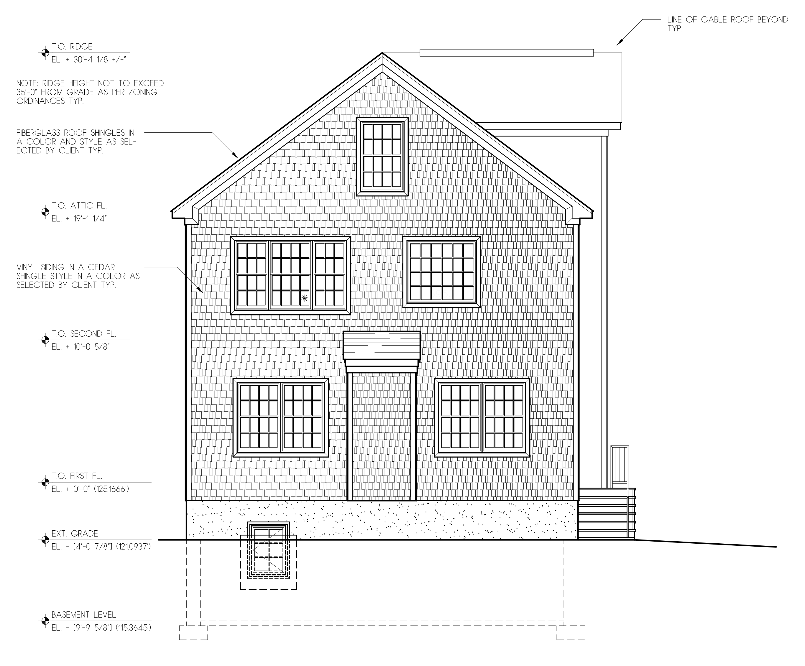
1 PROPOSED REAR YARD BUILDING ELEVATION SCALE: 1/4" = 1'-0"
