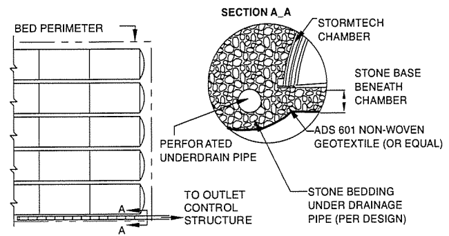
Figure 10 - Underdrain Parallel
