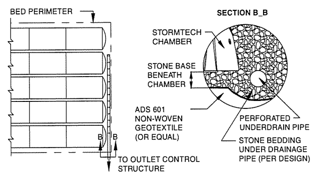
Figure 11 - Underdrain Perpendicular
