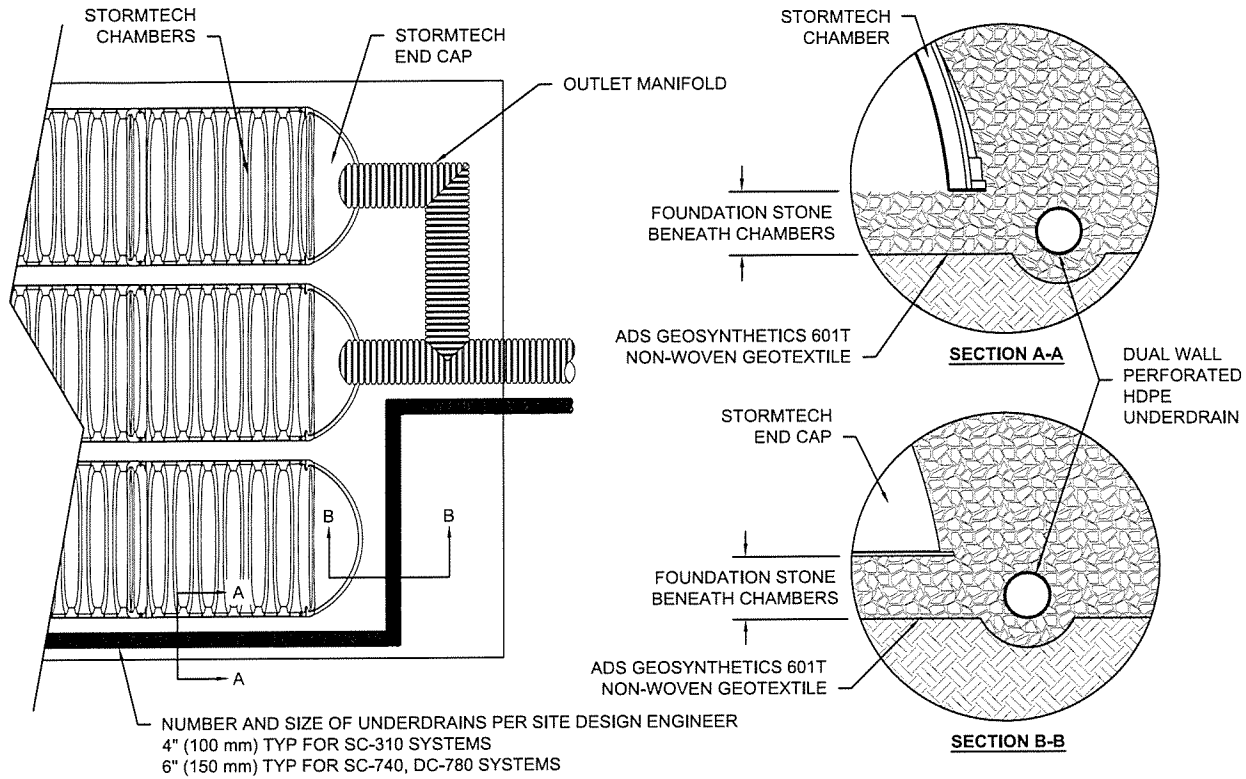
Figure 18 – Under Drain Detail
