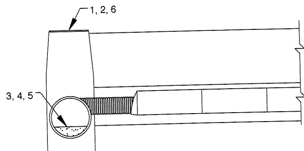
Figure 21 - Eccentric Manifold Maintenance
