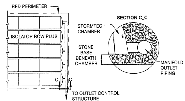
Figure 12 - Outlet Manifold
