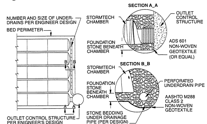
Figure 13 - Combination Outlet
