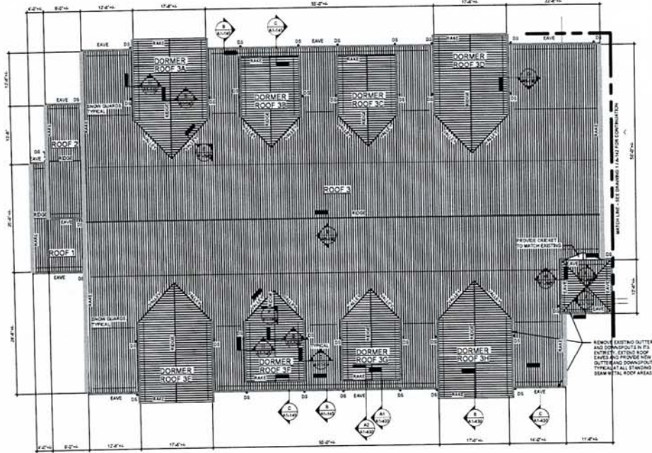
1 PARTIAL ROOF PLAN - ADMINISTRATION AREA SCALE: 1/8" = 1'-0"
