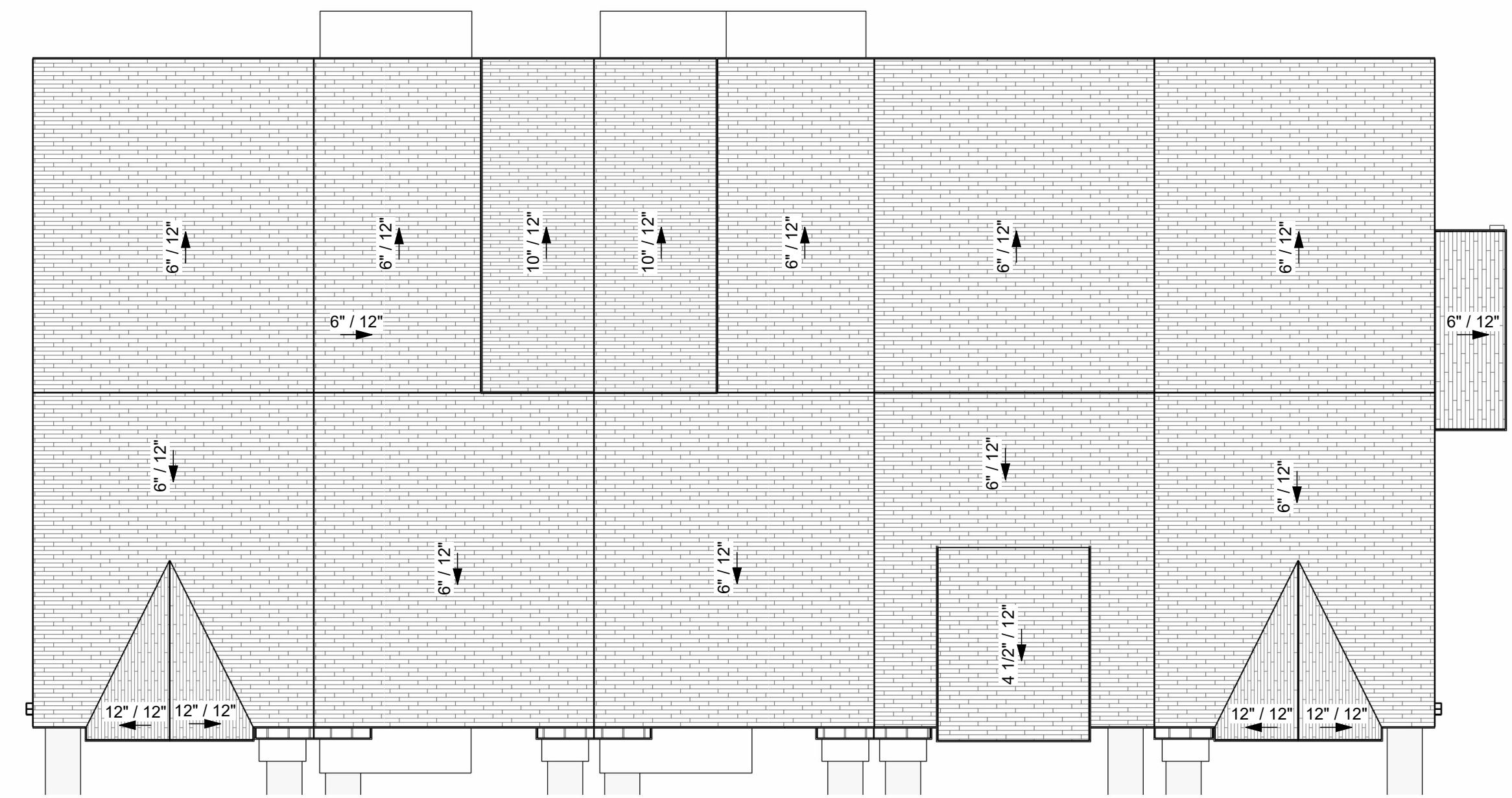
ADU & MARKET RATE ROOF PLAN
