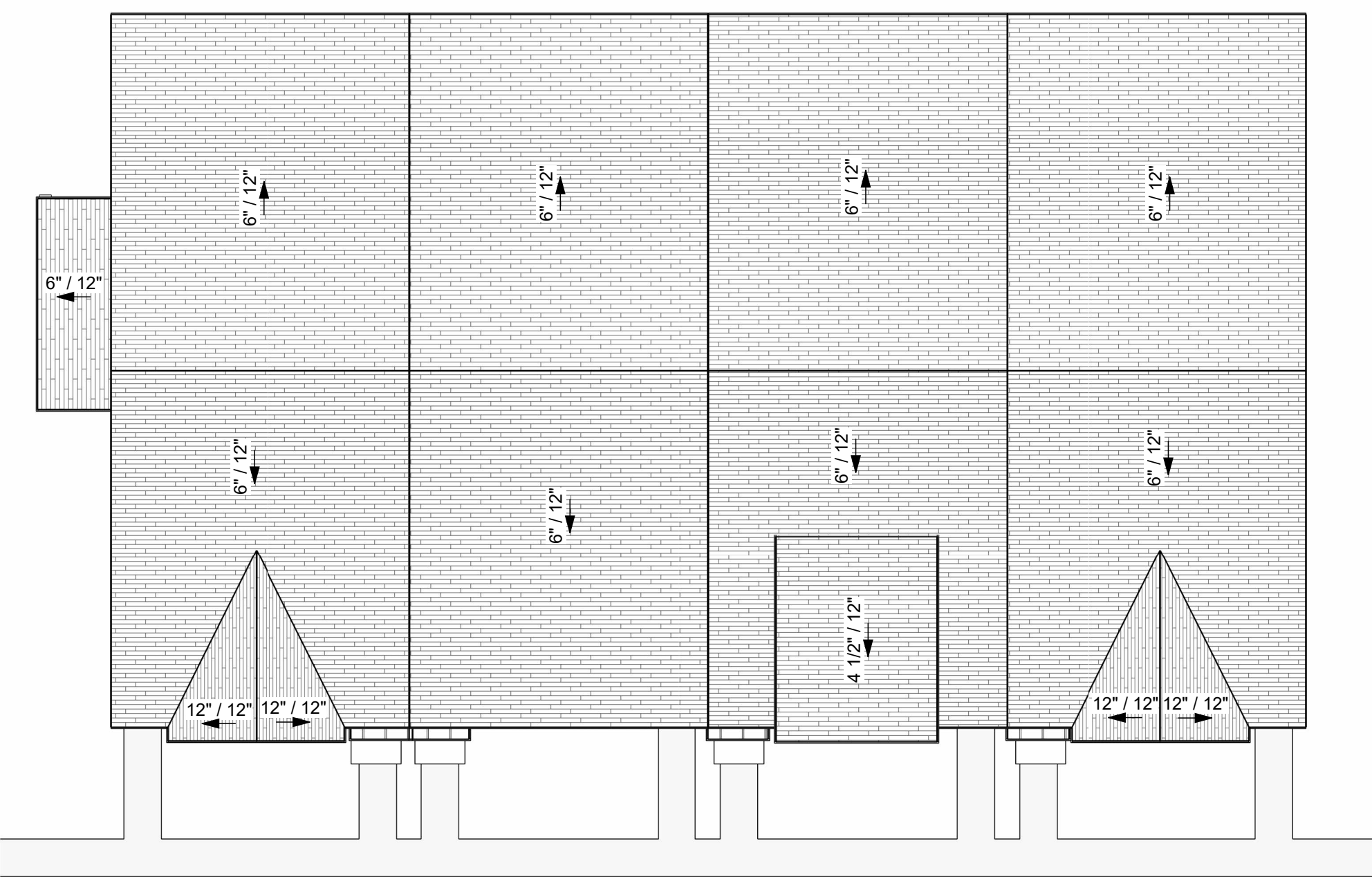
MARKET RATE ROOF PLAN
